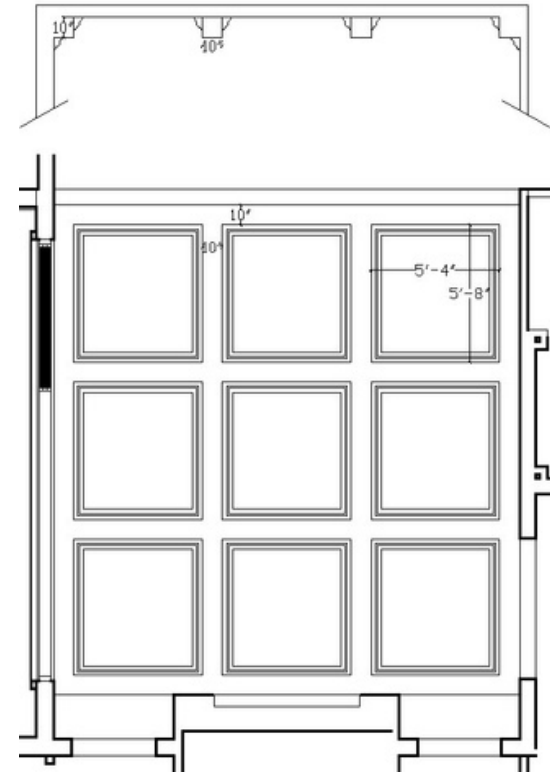
10" Square Drywall Beam Coffers & Crown
