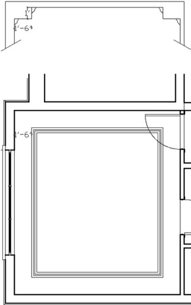
18" wide, 12" Deep Perimeter Soffit W/ Crown Accent paint
